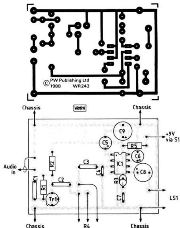
Fig. 3: Full size p.c.b. track pattern and component placement diagram of audio amplifier stage
