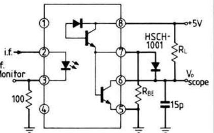
Fig. 2.6: An optocoupler speed-up circuit
