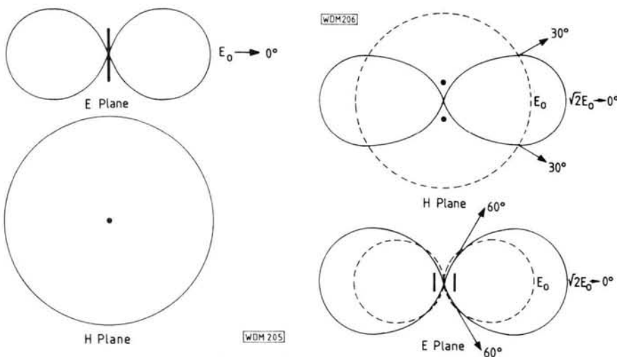
Fig. 5.1: Radiation patterns for a half wavelength dipole
