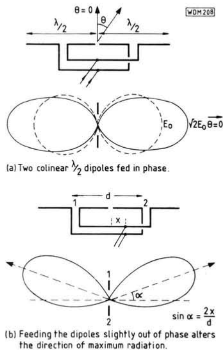
Fig. 5.4: Two collinear dipoles fed in phase have a gain of 2 in the E plane and a pattern which is identical to that of a full wave dipole. The direction of maximum radiation can be altered by moving the feed point
