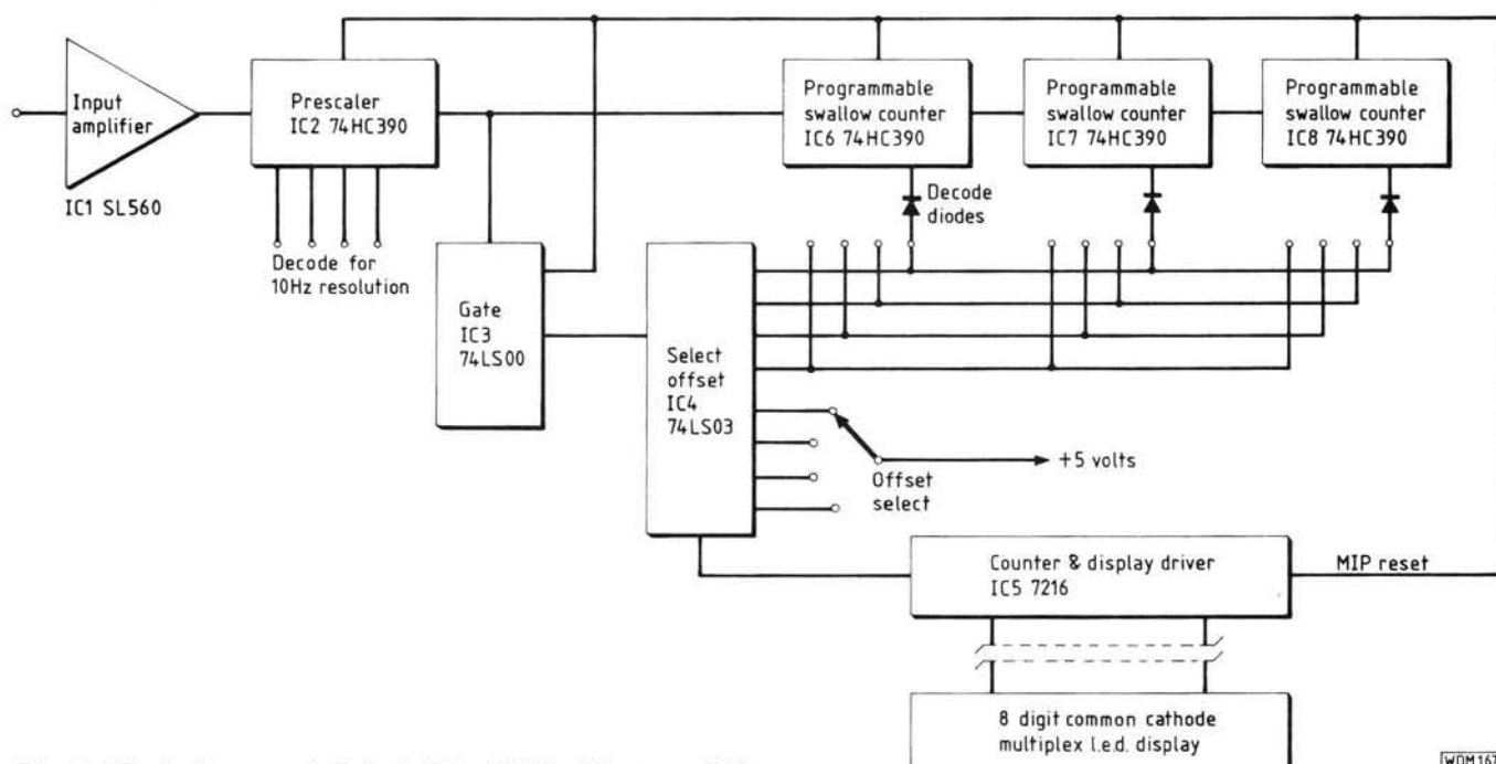
Fig. 1: Block diagram of digital dial with i.f. offset capability
