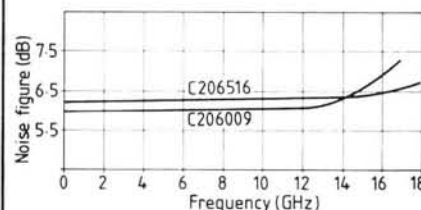
Fig. 2.1: Noise figure against frequency for the C206009 and C206516 devices
