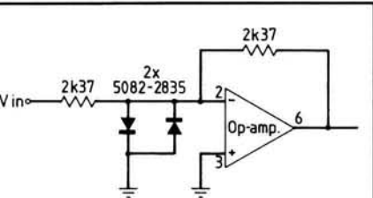
Fig. 2.5: Protecting an op-amp input with Schottky diodes
