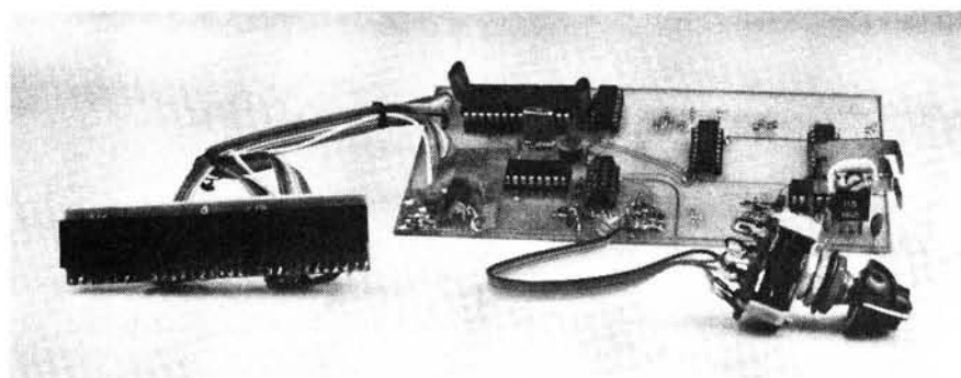
Digital dial prototype, note that IC1,2 must not be mounted in sockets as this will affect their h.f. performance
