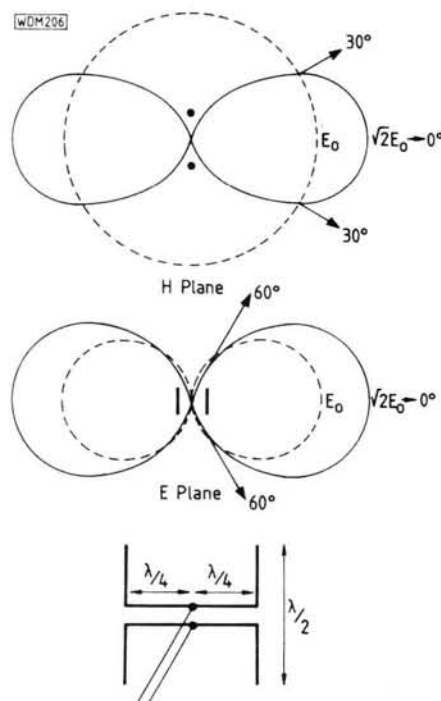
Fig. 5.1: Radiation patterns for a half wavelength dipole
